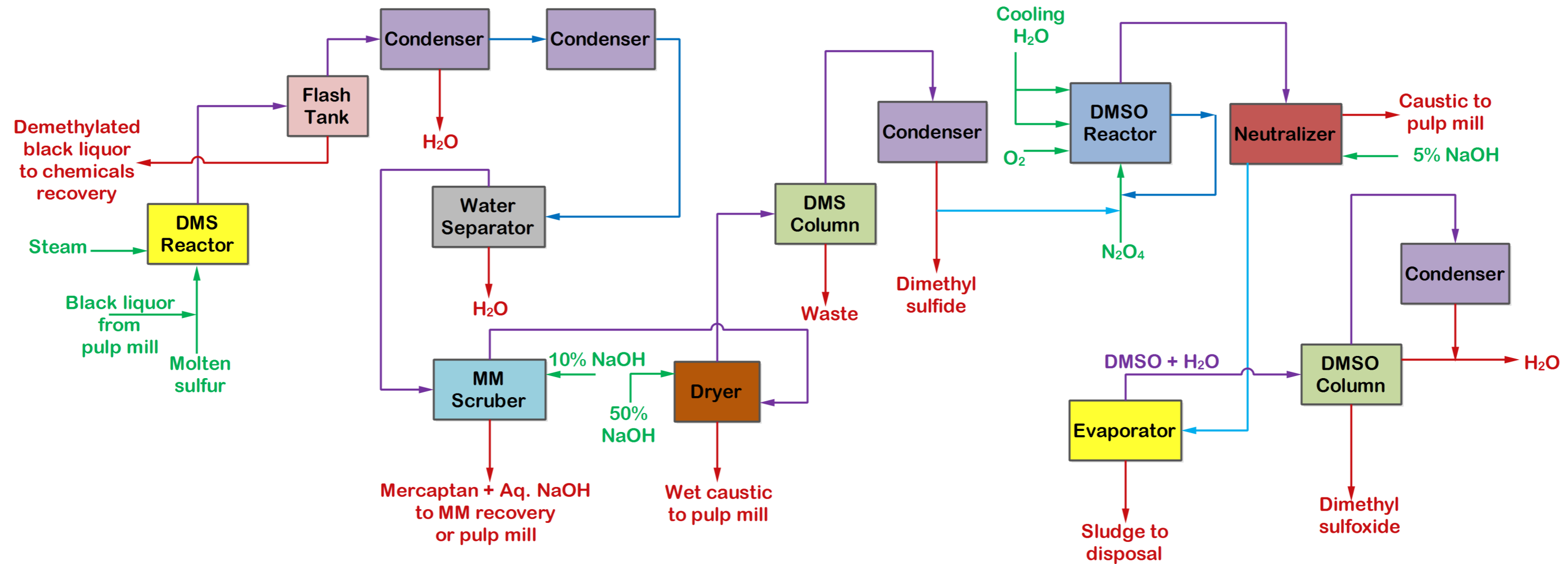
Figure: Manufacture of Dimethyl sulfoxide from wood liquor
